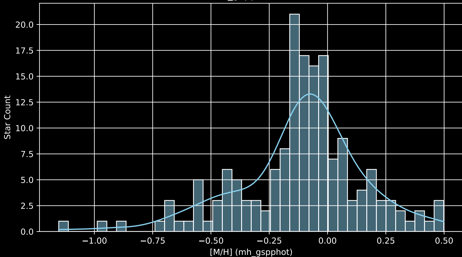
APOGEE DR17 Field: [165+18 [M/H] (mh_gspphot) (n= 166)
