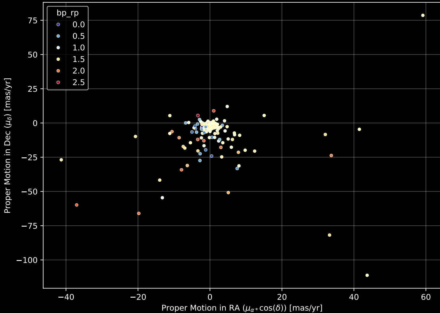
APOGEE DR17 Field: [165+18] Proper Motion Diagram (n= 167)
