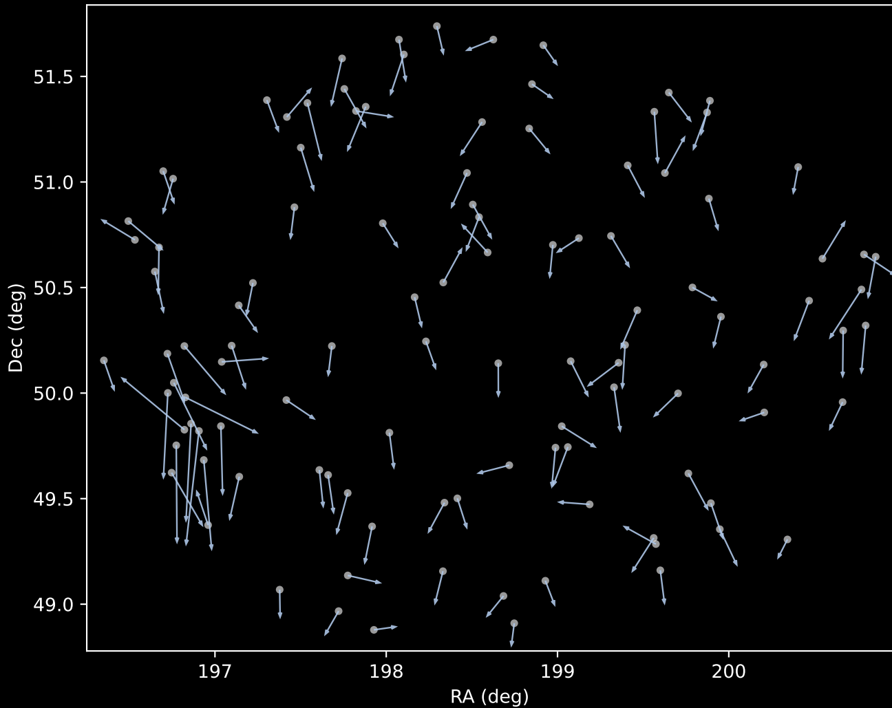
APOGEE DR17 Cluster 1 Proper Motion Vectors (n=109)
