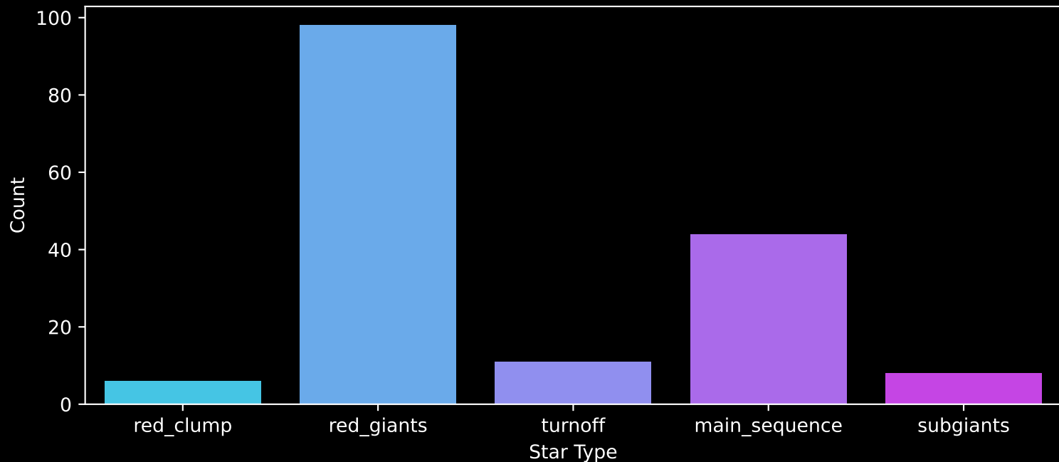
APOGEE DR17 Field: [165+18] Count plot of Star Type
