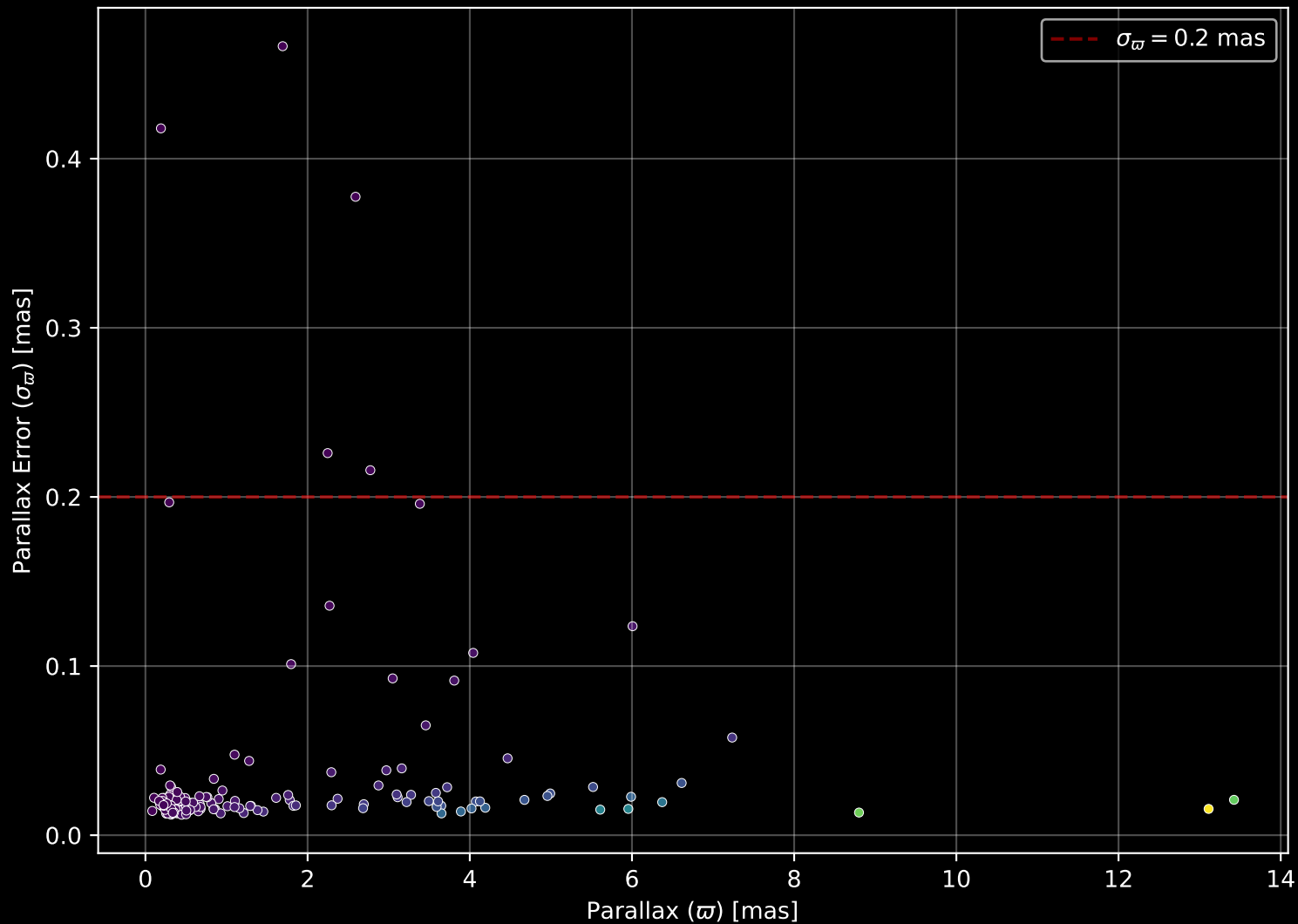
APOGEE DR17 Field: [165+18] Parallax Quality (n= 167)
