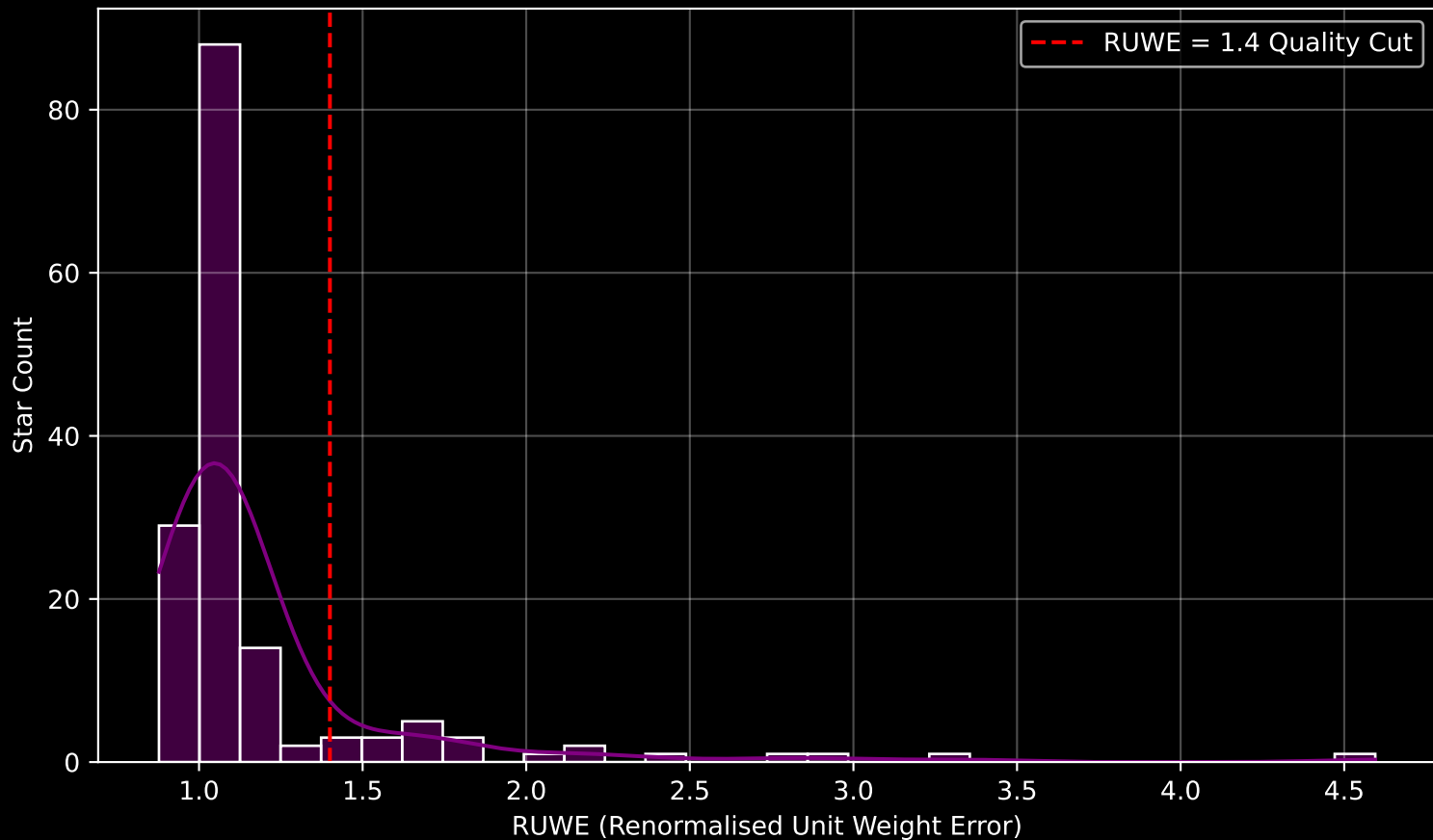
GAPOGEE DR17 Field [165+18] RUWE Distribution (n= 155)
